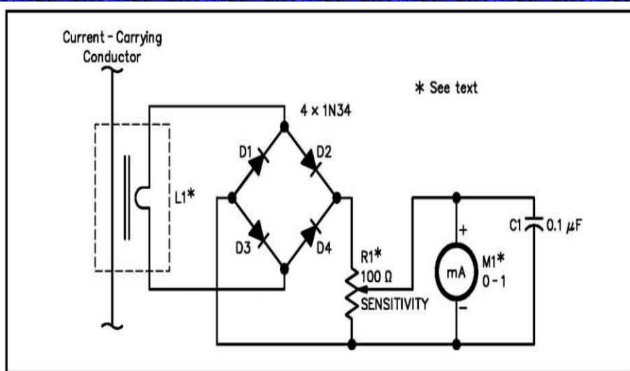
Figure 1—Schematic of the RF current probe. Unless otherwise specified, resistors are 1/4 W, 5% tolerance carbon-composition or film units. Part numbers in parentheses are RadioShack. Equivalent parts can be substituted.
